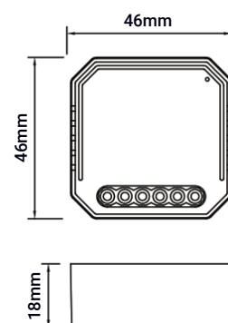
Bez klipsa / Without mounting clip
