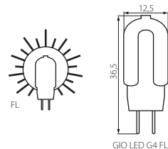
GIO LED G4 FL
