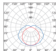
MIRA 2 × 18W
