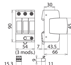
Dimension drawing DG MU SPN 240 3W+G R
