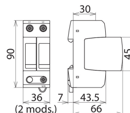
Dimension drawing DG MU SP 480 3W+G
