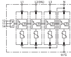
Basic circuit diagram DG MU 3PH 240 4W+G R
