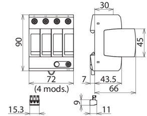
Dimension drawing DG MU 3PY 600 4W+G R
