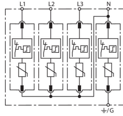
Basic circuit diagram DG MU 3PY 208 4W+G
