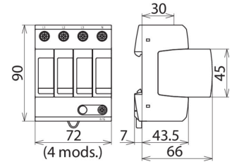
Dimension drawing DG MU 3PY 208 4W+G
