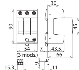
Dimension drawing DG MU 3PD 480 3W+G R
