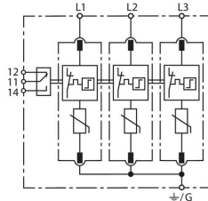
Basic circuit diagram DG MU 3PD 480 3W+G R
