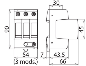
Dimension drawing DG MU 3PD 240 3W+G
