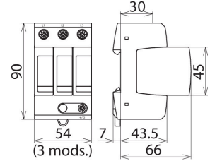
Dimension drawing DG MU 3PD 480 3W+G
