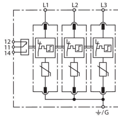
Basic circuit diagram DG MU 3PY 600 3W+G R
