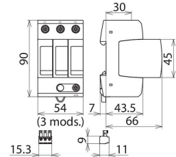
Dimension drawing DG MU 3PY 480 3W+G R
