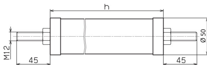
Dimension drawing DMI 30 10 1 L
