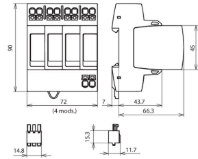
Dimension drawing DG MP TNS 150 FM
