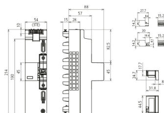
Dimension drawing DSH ZP 2 LSG A TT 255
