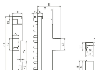
Dimension drawing DSH ZP B2 TNS 255
