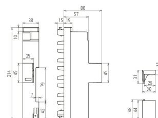
Dimension drawing DSH ZP 2 TNS 255
