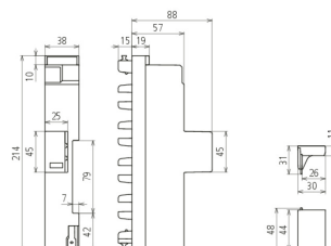
Dimension drawing DSH ZP B2 TT 255
