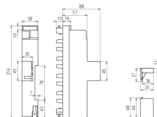
Dimension drawing DSH ZP 2 TT 255
