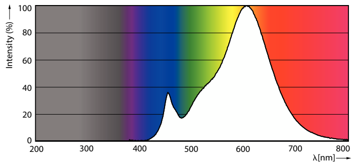
Spectral Power Distribution Colour - PILA LED 75W A60 E27 WW FR ND 1CT/6 G3
