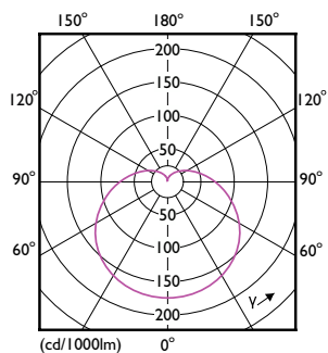
Light Distribution Diagram - PILA LED 75W A60 E27 WW FR ND 1CT/6 G3
