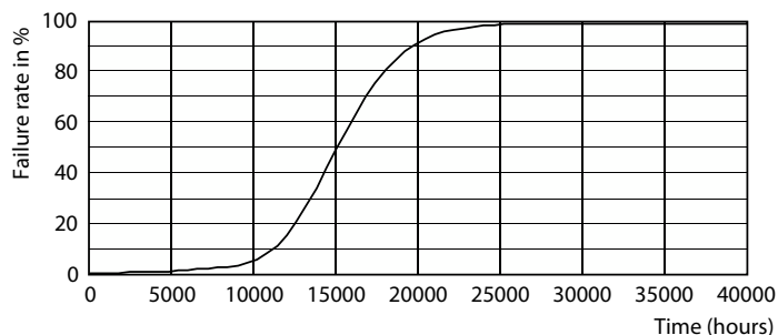
Life Expectancy Diagram - PILA LED 60W A60 E27 CW FR ND 1CT/6
