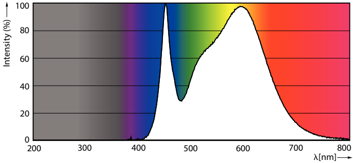
Spectral Power Distribution Colour - PILA LED 60W A60 E27 CW FR ND 1CT/6
