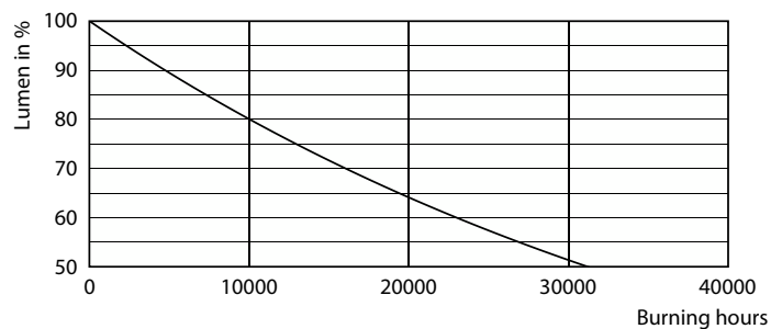
Lumen Maintenance Diagram - PILA LED 60W A60 E27 CW FR ND 1CT/6
