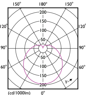
Light Distribution Diagram - PILA LED 60W A60 E27 CW FR ND 1CT/6
