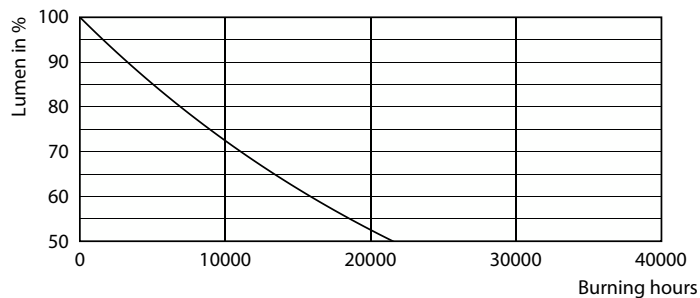
Lumen Maintenance Diagram - PILA LED 60W A60 E27 WW FR ND 1CT/6
