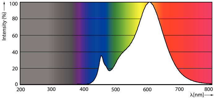
Spectral Power Distribution Colour - PILA LED 60W A60 E27 WW FR ND 1CT/6
