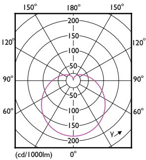
Light Distribution Diagram - PILA LED 60W A60 E27 WW FR ND 1CT/6
